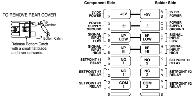
REAR VIEW OF CASE AND CONNECTOR
